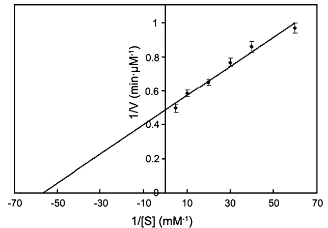
Fig. 4 Lineweaver-Burk plot for kinetics determinations of purified SaALDC using \alpha -acetolactate as the substrate
